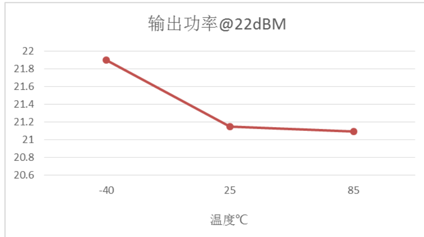
Figure 3-4 max TXOP vs Temperature (470MHz)
