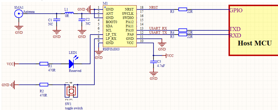
Figure 4-3 Reference design with RHF0M003-XF22
