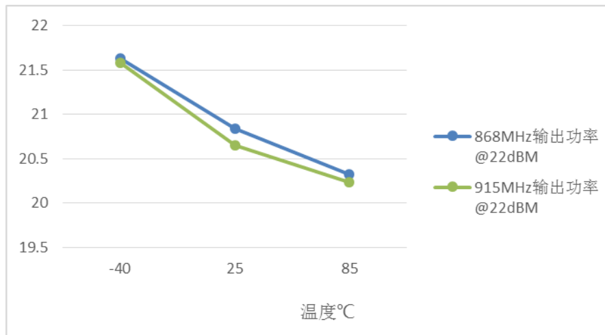
Figure 3-10 max TXOP vs Temperature (868/915MHz)
