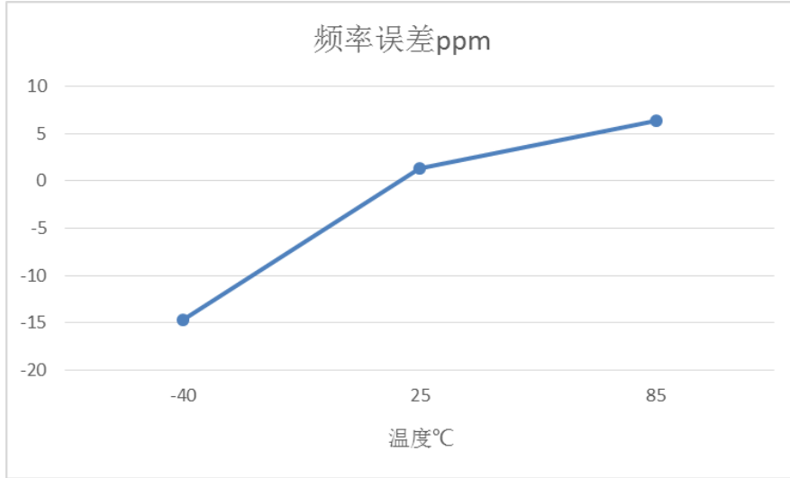
Figure 3-3 Frequency Tolerance vs Temperature (470MHz)
