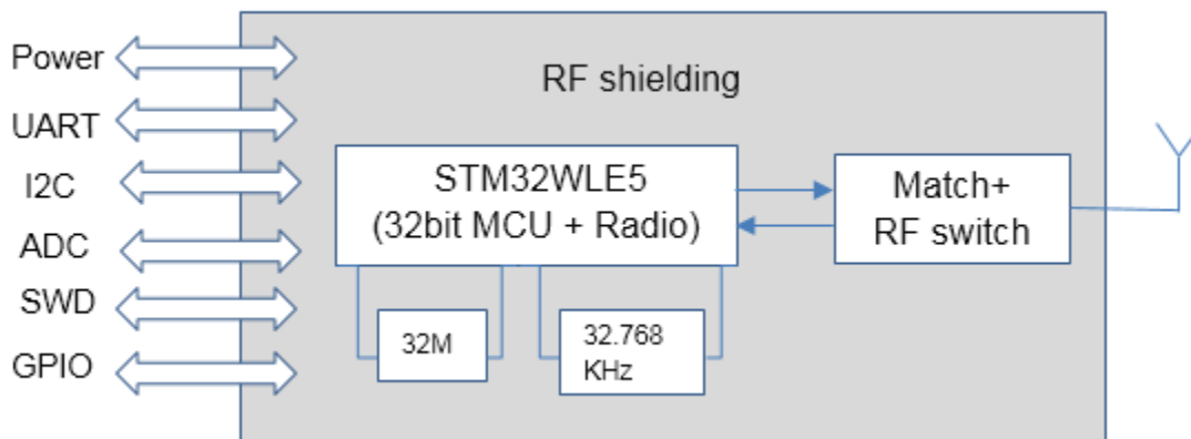
Figure 1-1 Block Diagram of RHF0M003-XF22
