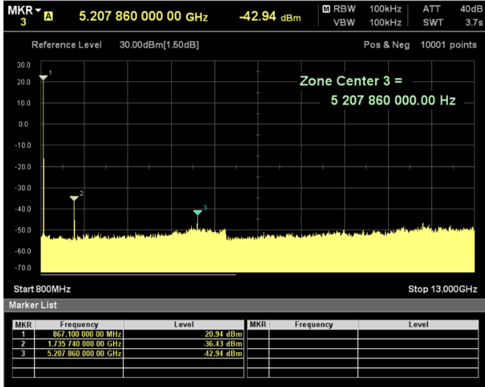
Figure 3-12 Harmonics measurement @Frf=868MHz, TXOP=22dBm
