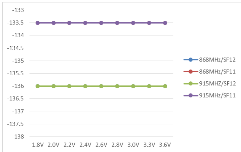
Figure 3-8 Sensitivity (SF11/SF12,125kHz) vs Supply voltage (868/915MHz)
