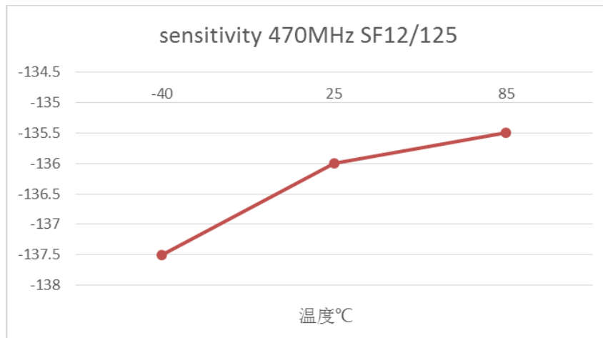
Figure 3-5 Sensitivity (SF12,125kHz) vs temperature
