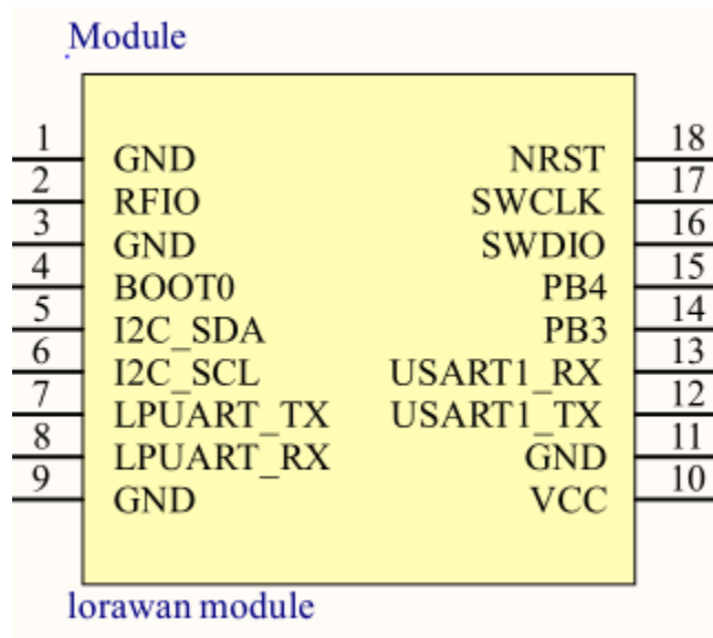
Figure 1-2 schematic of RHF0M003-XF22
