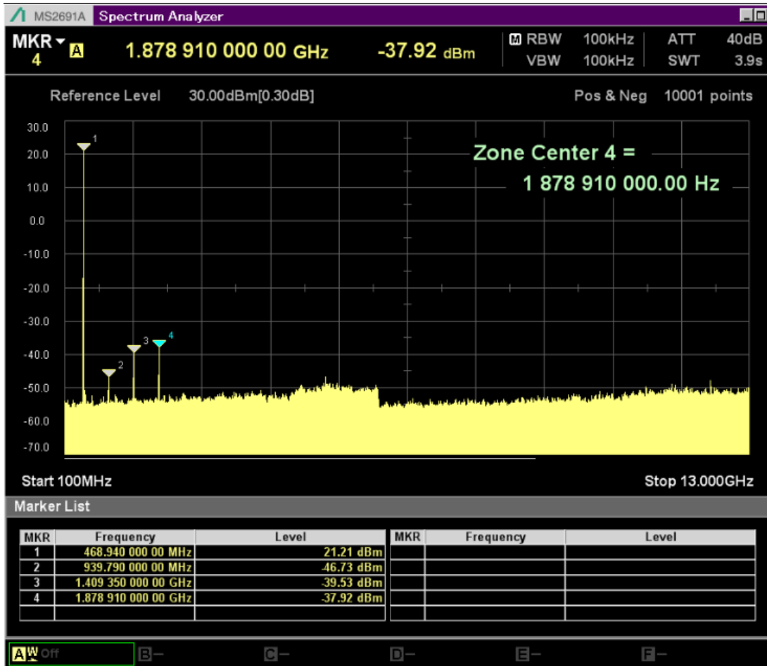
Figure 3-6 Harmonics measurement @Frf=470MHz, TXOP=22dBm
