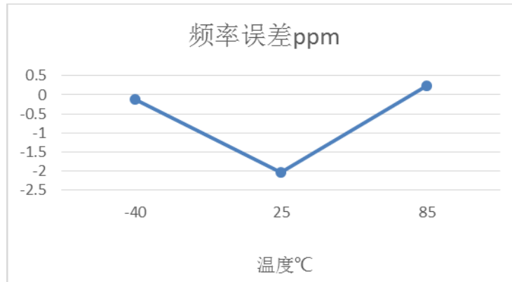
Figure 3-9 Frequency Tolerance vs Temperature
