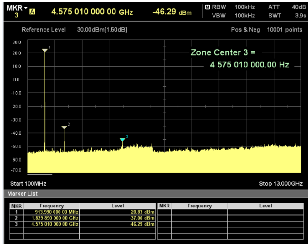
Figure 3-13 Harmonics measurement @Frf=915MHz, TXOP=22dBm
