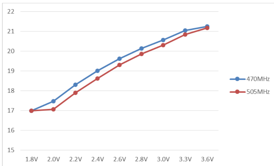
Figure 3-1 max TXOP vs Supply voltage
