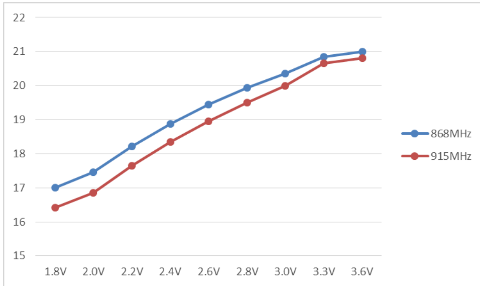
Figure 3-7 max TXOP vs Supply voltage (868/915MHz)
