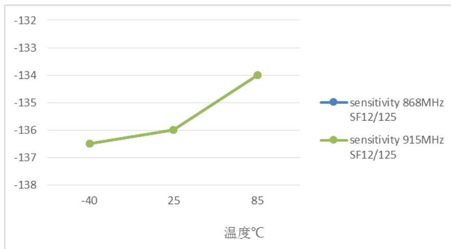
Figure 3-11 Sensitivity (SF12,125kHz) vs temperature (868/915MHz)
