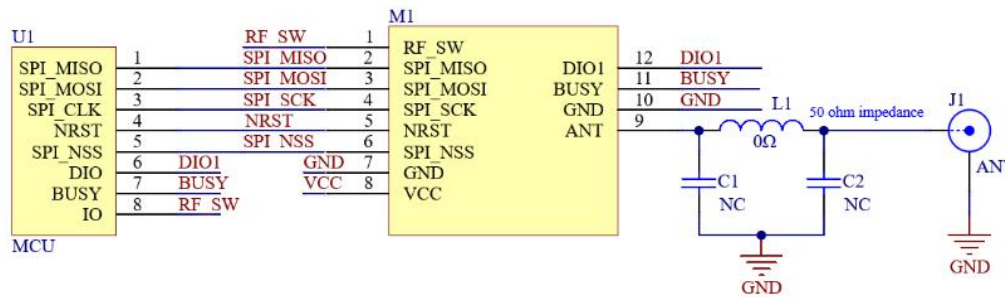
Figure 14 Reference design based on RHF0M62H
