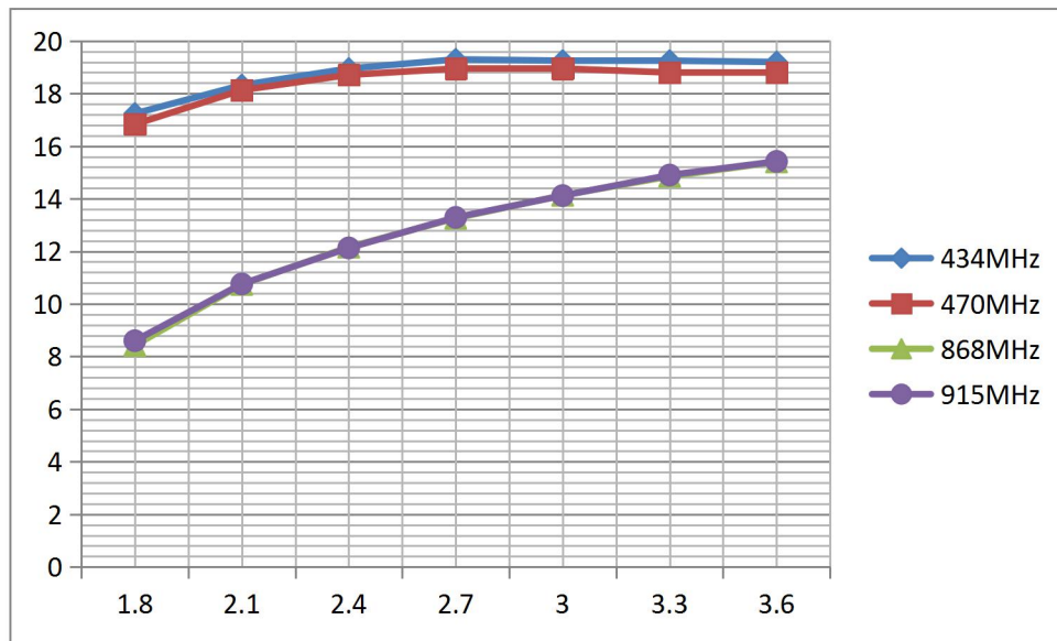
Figure 4 TXOP vs Supply voltage
