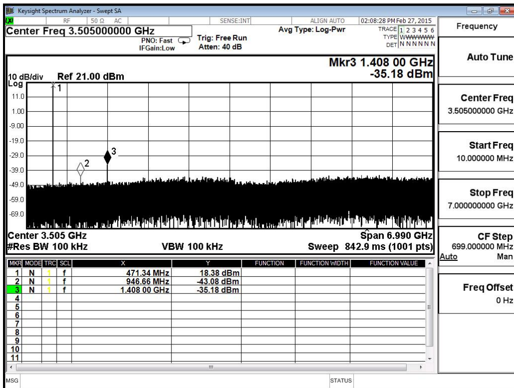
Figure 10 Harmonics measurement @Frf=470MHz, TXOP=19dBm
