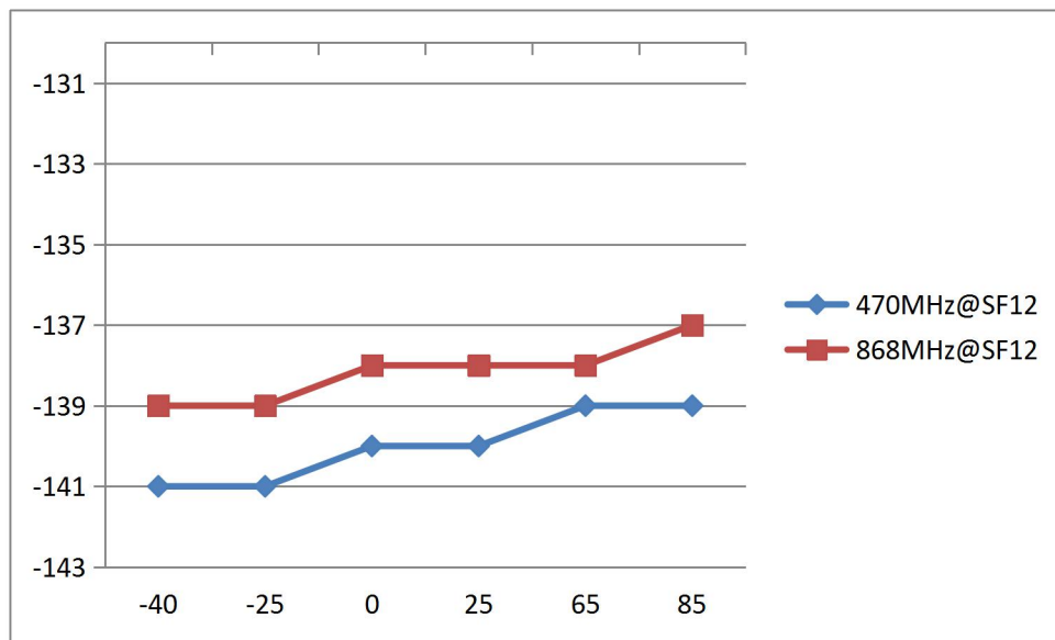
Figure 8 Sensitivity (SF12,125kHz) vs temperature
