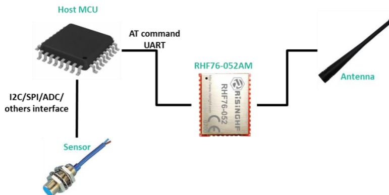
Figure 19 LoRaWAN sensor with RHF76-052DM
