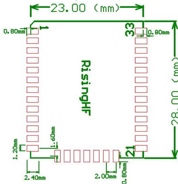
Figure 14 Recommended land pattern
