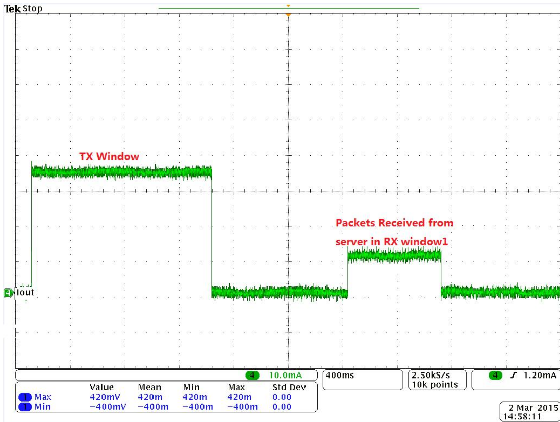
Figure 18 Energy profile of RHF76-052 application in LoRaWAN (A packet received from Server in RX window1)
