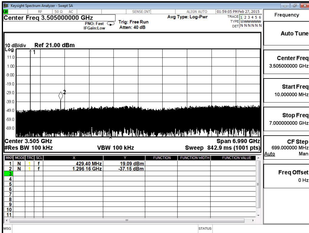
Figure 9 Harmonics measurement @Frf=434MHz, TXOP=19dBm
