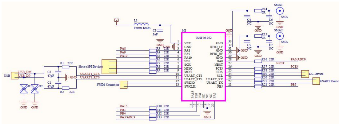
Figure 16 Reference design with RHF76-052
