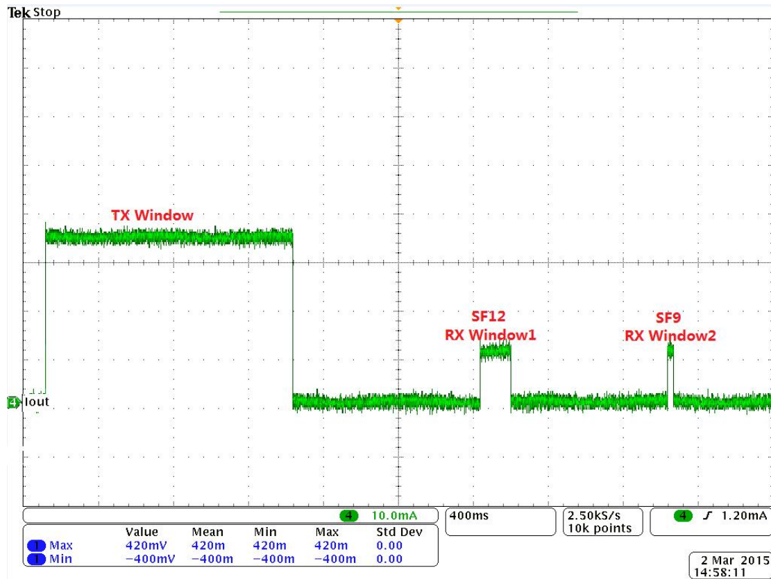
Figure 17 Energy profile of RHF76-052 application in LoRaWAN (No packet received from Server)
