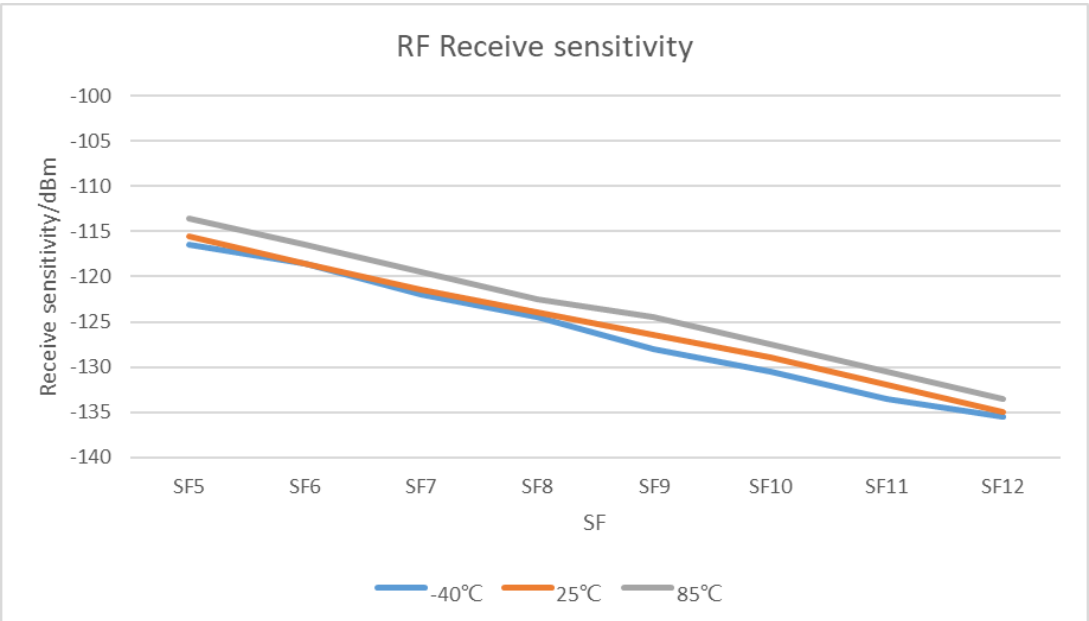
Figure 15 RF Receiver Sensitivity VS Temperature (915MHz)
