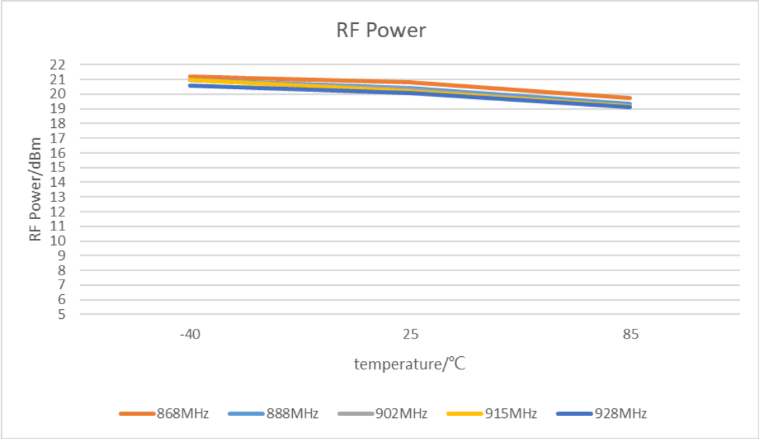
Figure 12 RF Power VS Temperature (868~928MHz)
