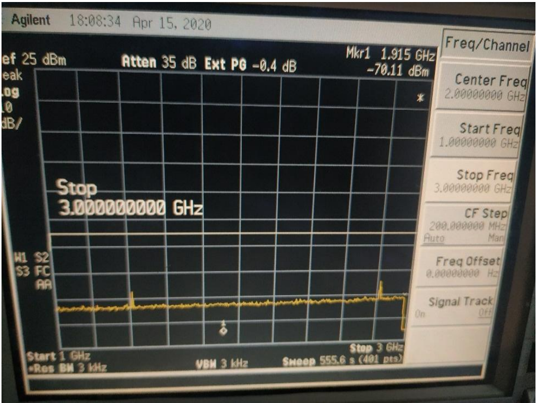
Figure 8 Harmonic(1GHz~3GHz)@Fr f =470MHz, TXOP=22dBm
