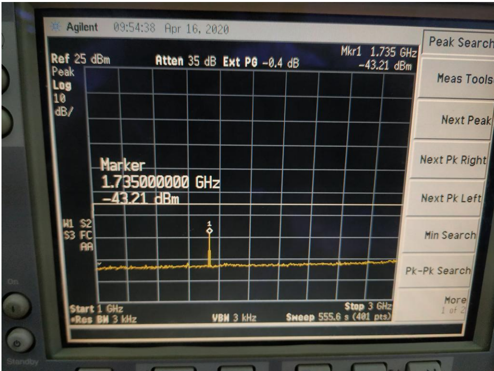
Figure 17 Harmonic(1GHz~3GHz)@Frf=868MHz, TXOP=22dBm
