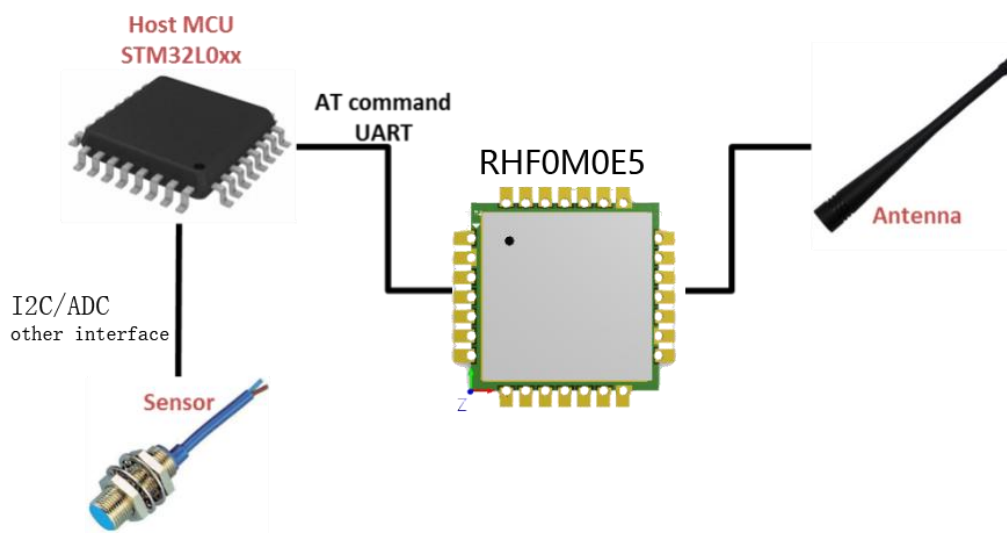
Figure 21 Design of LoRaWAN® wireless sensor based on RHF0M0E5 module
