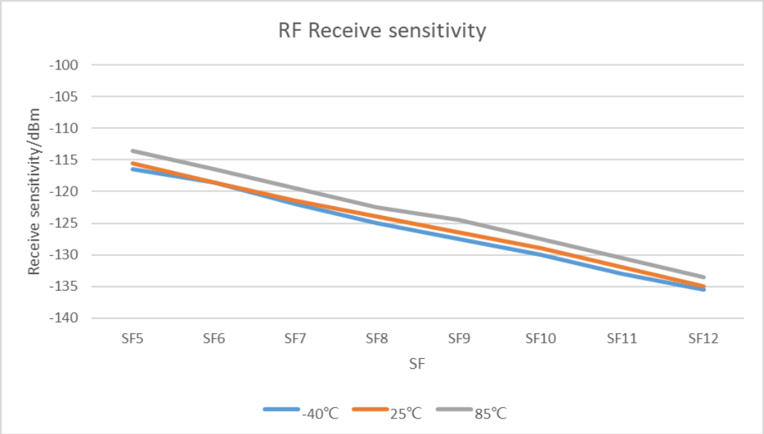
Figure 14 RF Receiver Sensitivity VS Temperature (868MHz)
