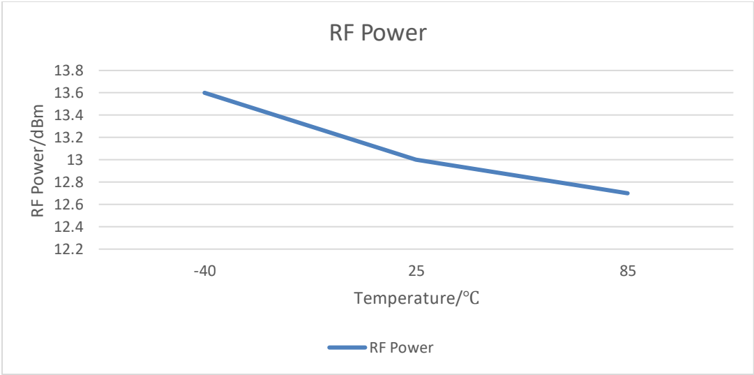
Figure 10 RF Power VS Temperature（868MHz）only for RHF0M0E5-HF14
