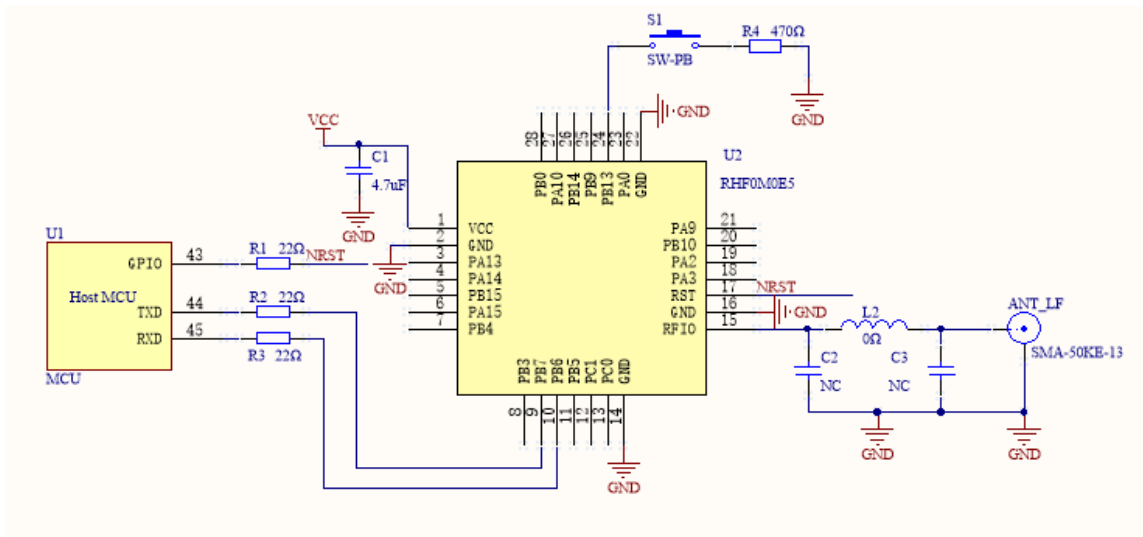
Figure 20 Reference design based on RHF0M0E5
