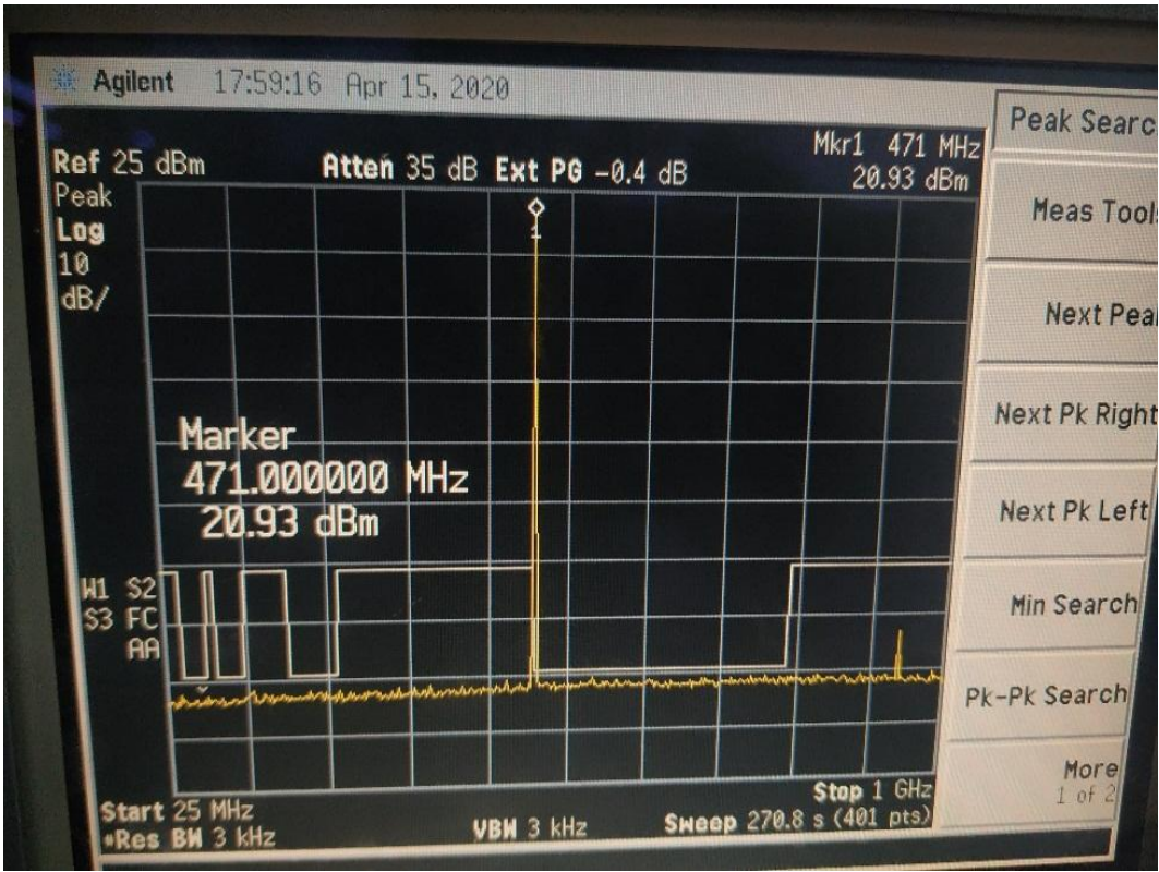
Figure 7 Harmonic(25MHz~1GHz)@Frf=470MHz, TXOP=22dBm
