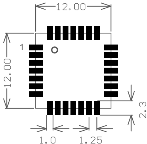
Figure 19 PCB footprint
