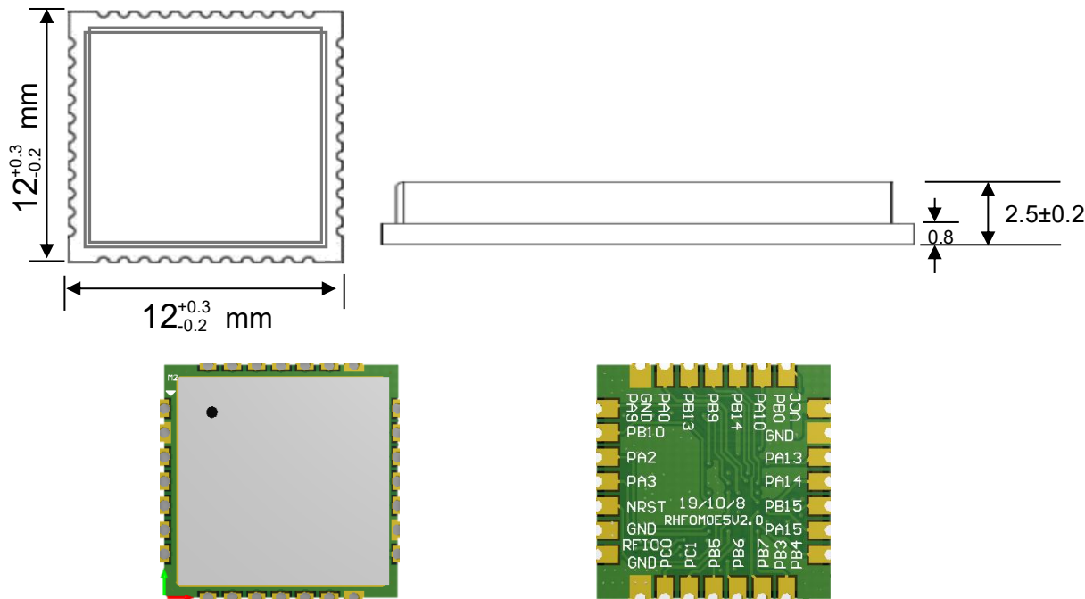
Figure 18 RHF0M0E5 Module appearance
