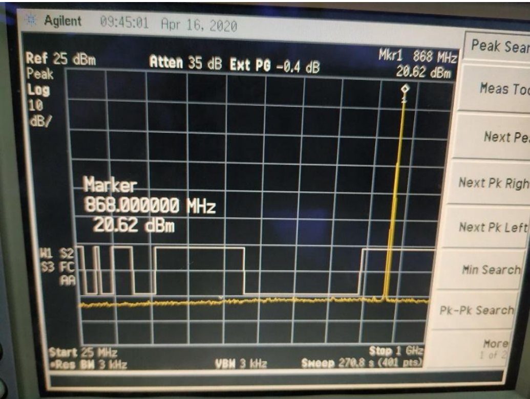
Figure 16 Harmonic(25MHz~1GHz)@Frf=868MHz, TXOP=22dBm
