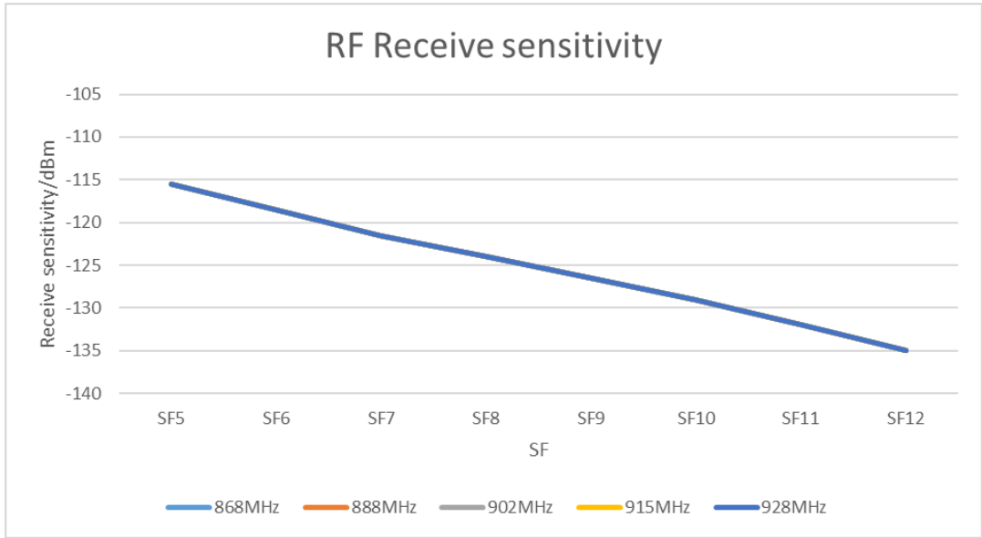
Figure 13 RF Receiver Sensitivity vs Spreading factor (868~928MHz)
